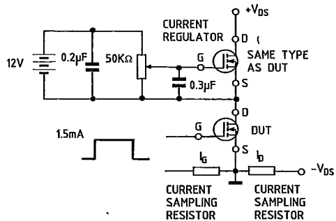
Gate charge test circuit
