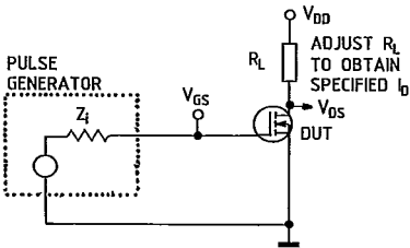
Switching times test circuit
