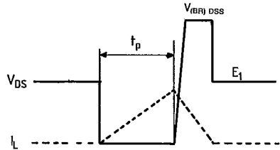
Unclamped inductive waveforms
