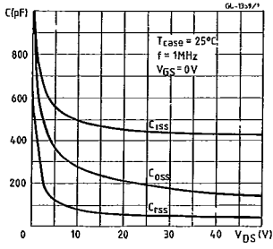
Capacitance variation
