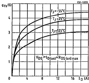
Transconductance
