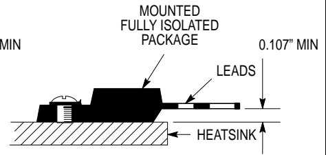
Figure 17. Screw Mounting Position for Isolation Test Number 3
