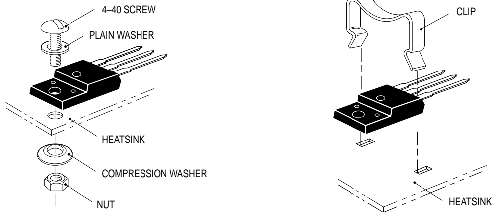
Figure 18. Typical Mounting Techniques for Isolated Package
