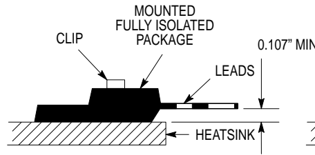
Figure 16. Clip Mounting Position for Isolation Test Number 2
