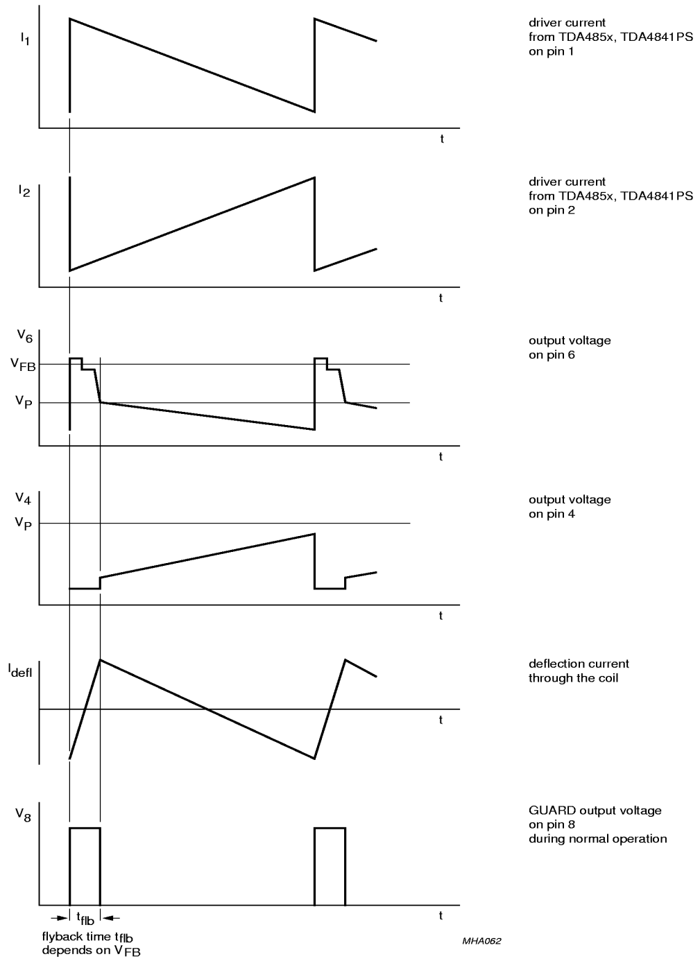
Fig.5 Timing diagram.
